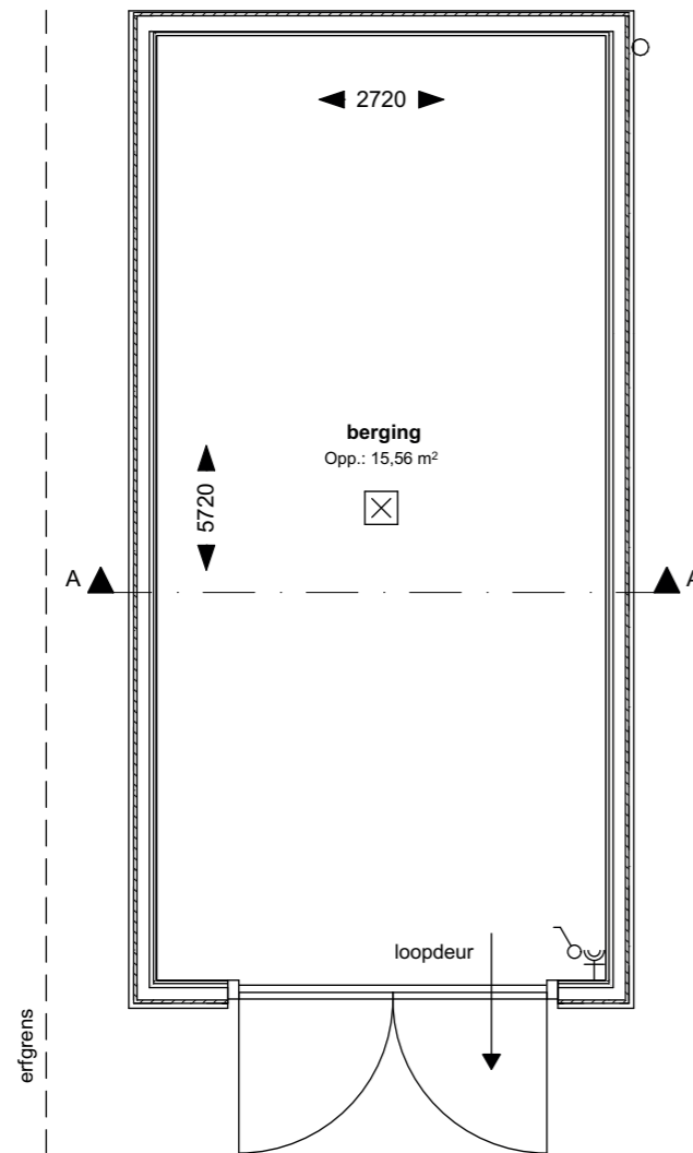
1:50 00 Begane grond
