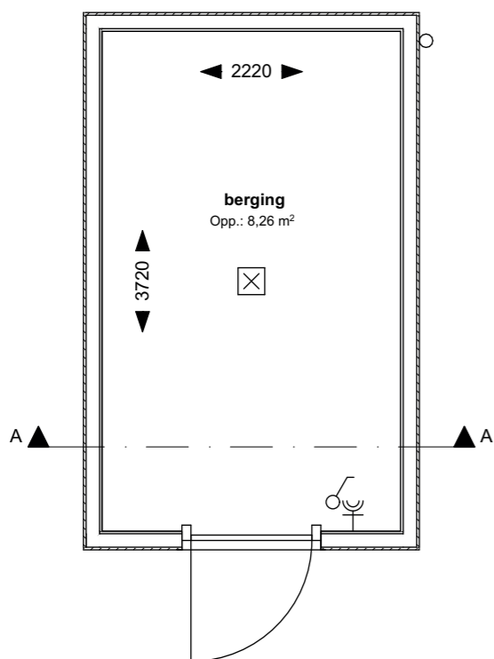
1:50 00 Begane grond
