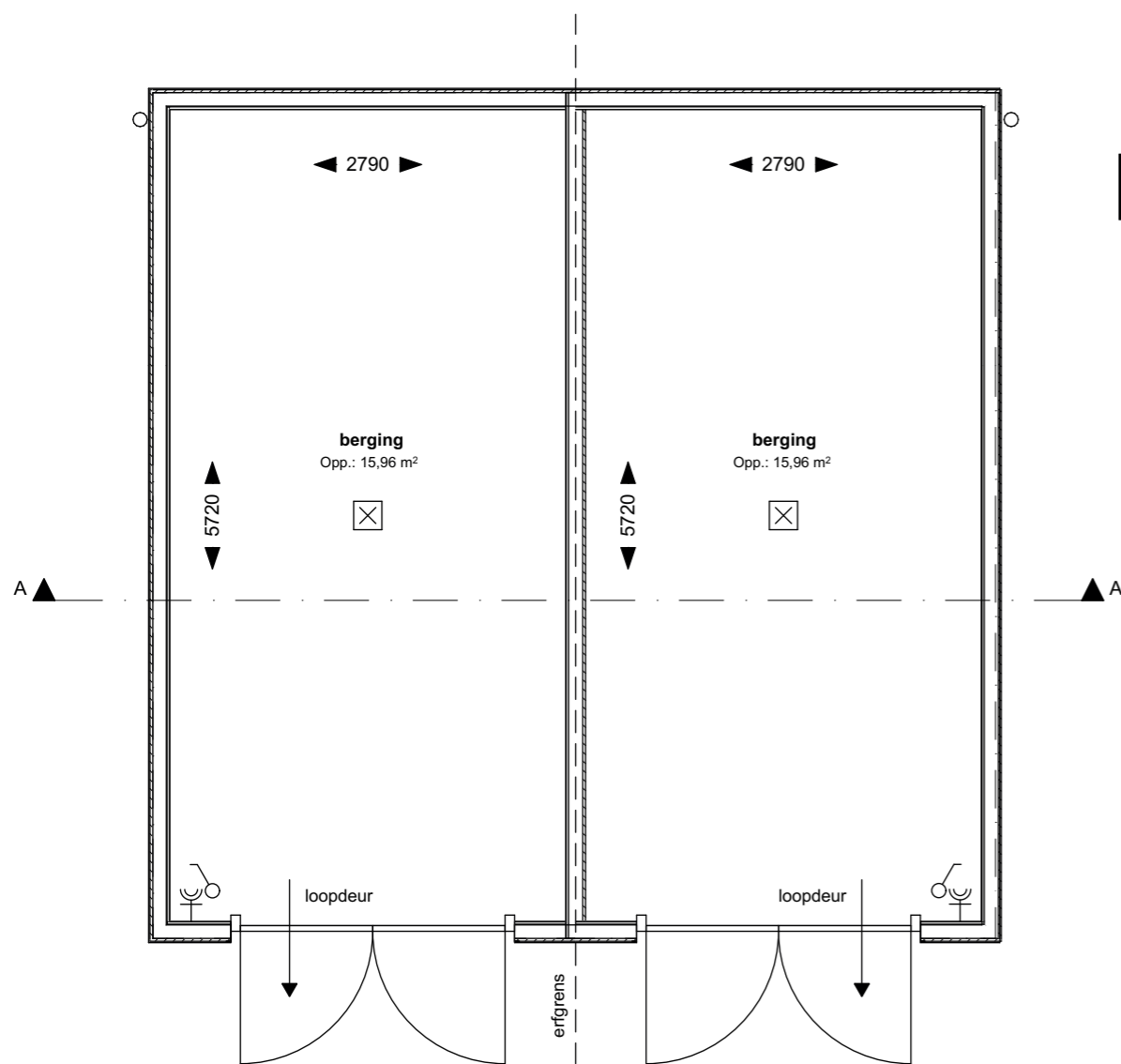
1:50 00 Begane grond
