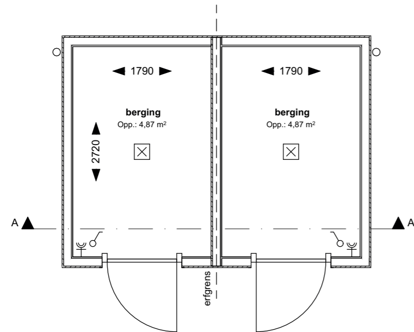
1:50 00 Begane grond
