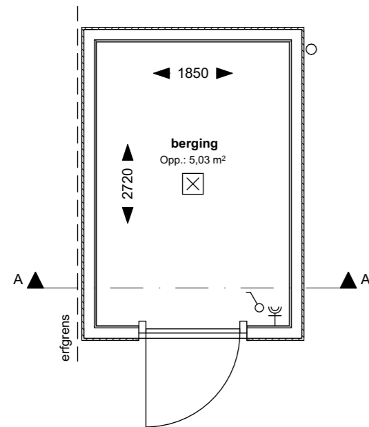
1:50 00 Begane grond
