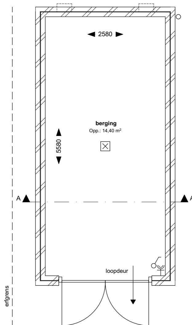
1:50 00 Begane grond
