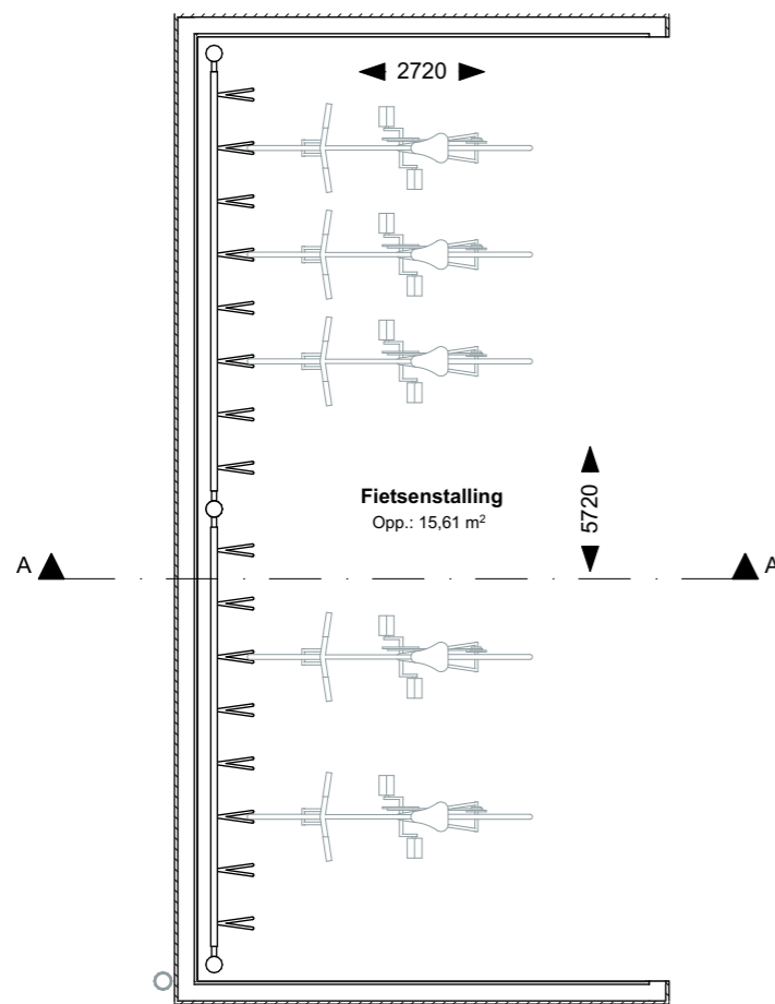
1:50 00 Begane grond
